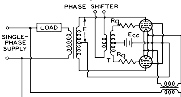
FIG. 4 FULL-WAVE SINGLE-PHASE
