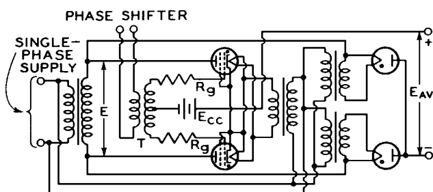
FIG. 3 SERIES SINGLE-PHASE
