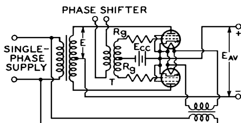
FIG. 2 FULL-WAVE SINGLE-PHASE
