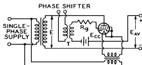
FIG. 1 HALF-WAVE SINGLE-PHASE
